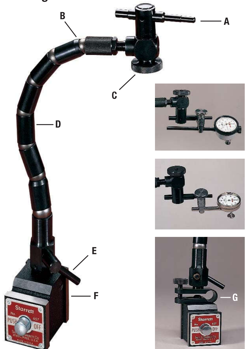
Top inset, No. 651B1 Indicator gripped directly to its stem via the post snug; middle, holding a No. 196B1 Indicator via a No. 657S Snug attached to the indicator's 1/4" (6.3 mm) diameter rod; bottom, No. 657W Fine-Adjustment Attachment.
